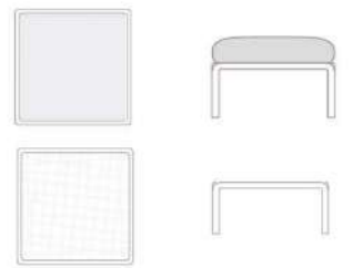
DIMENSIONS / CM: PUFF: L 70 D 70 H 32
